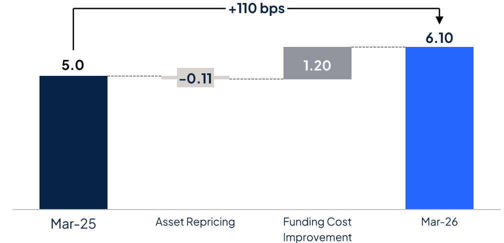
NIM 1 Evolution
